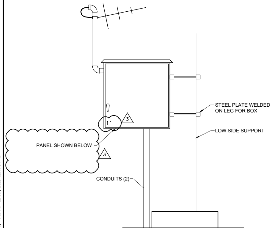
ANTENNA INSTALLATION DETAIL
